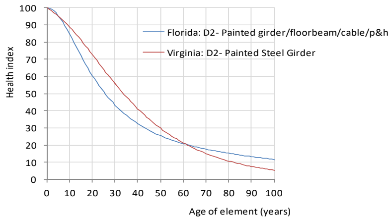
Exhibit 28: Examples of Bridge Deterioration Models
