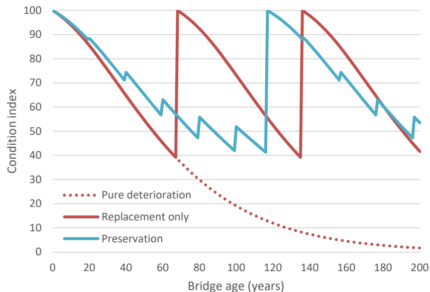
Exhibit 47: Preservation Extends the Service Life of a Typical Alabama Bridge
